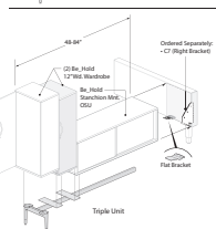
BAES Legs - Single, Double or Triple Unit for use with Compose Connections
