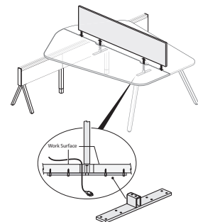
Half Convergent Adaptable Worksurfaces
