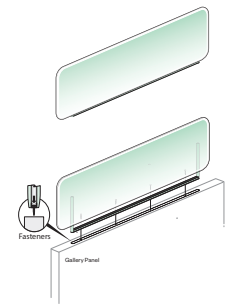
Accessory Frame – Fabric for use with Gallery Panels
