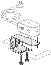
Knife Edge Worksurface Mount
