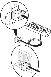
Circuit Breaker Plug Detail Class YA
