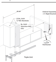
BAES Legs - Single, Double or Triple Unit for use with Compose Connections
