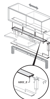
For use with Compose 26" (660mm) High Panel, Compose Connections and Compose Beam — Off-Modular Rail Mounting — Off-Modular Rail for mounting Compose to Be_Hold Upper Storage — Stanchion Mounted
