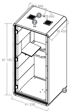
1 Cutout for sprinkler installation 2 Power cable access
