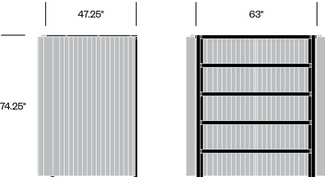
High Frame, 47.25" x 63"
