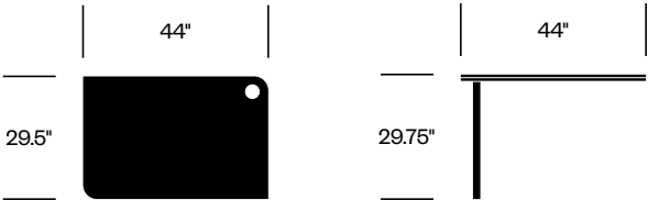
Worktop, 44" x 29.5" (Side A)
