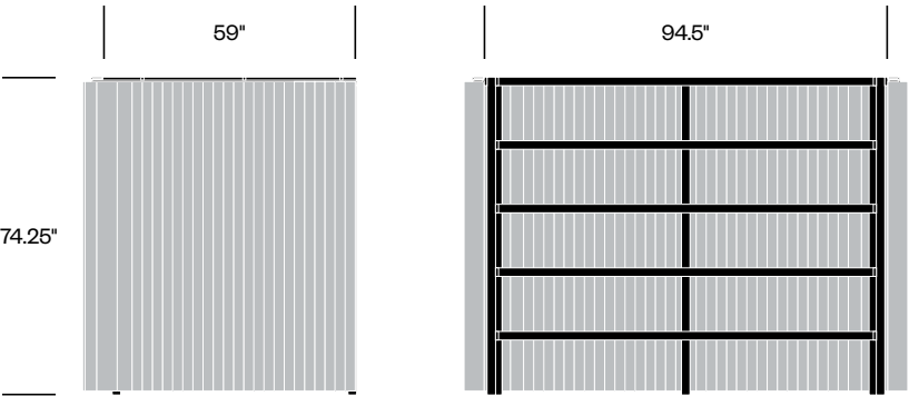
High Frame, 59" x 94.5"
