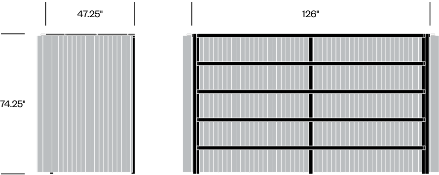
High Frame, 47.25" x 126"
