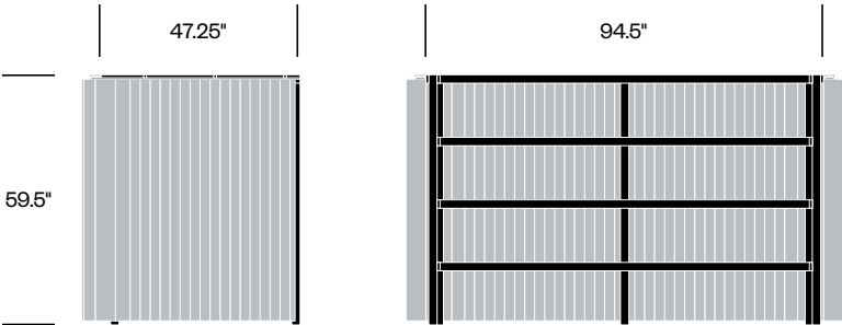
Medium Frame, 47.25" x 94.5"
