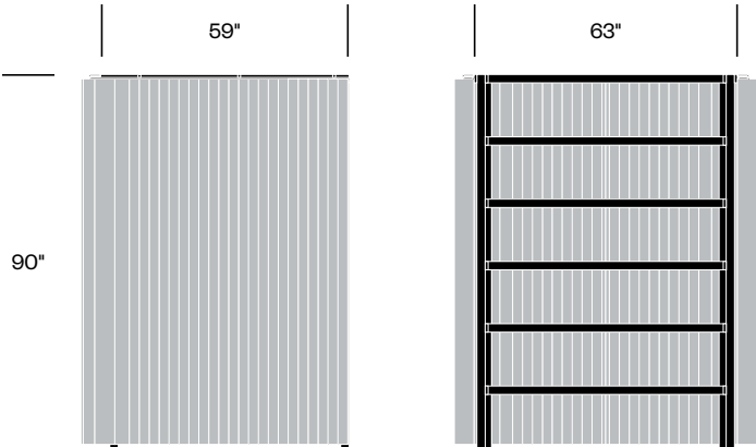
Extra High Frame, 59" x 63"
