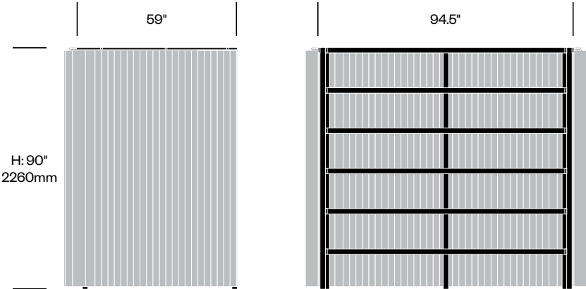
Extra High Frame, 59" x 94.5"
