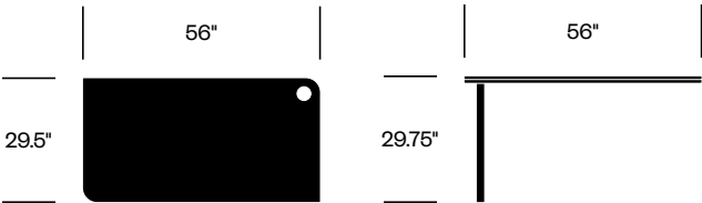
Worktop, 56" x 29.5" (Side A)
