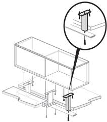
For use with Compose 26"(660mm)H Panel, Connections and Beam — Centered Single Panel Mount Stanchion for Aluminum Top Trim
