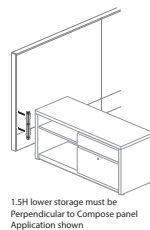
Compose Panel-to-Storage Bracket — C5 Be_Hold/A Series Credenza
