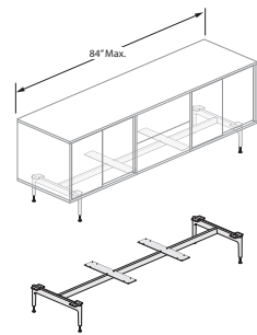
Legs — Triple Unit
